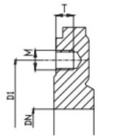
Blind hole tapping
